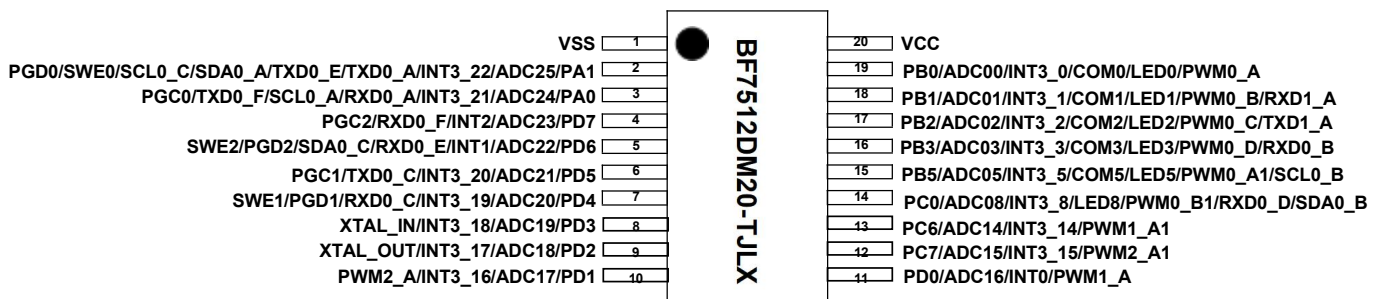
BF7512DM20-TJLX package pin diagram
