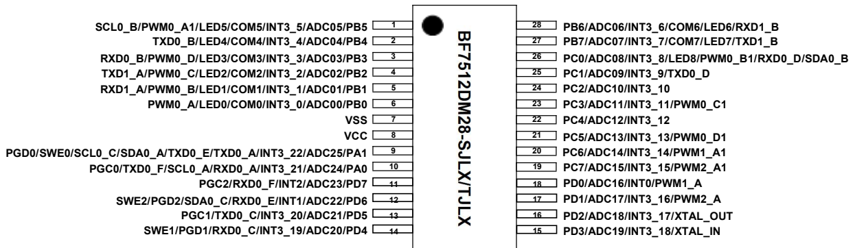
BF7512DM28-SJLX/TJLX package pin diagram
