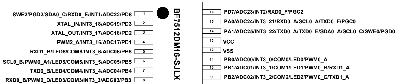
BF7512DM16-SJLX package pin diagram
