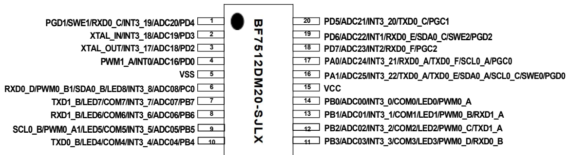
BF7512DM20-SJLX package pin diagram
