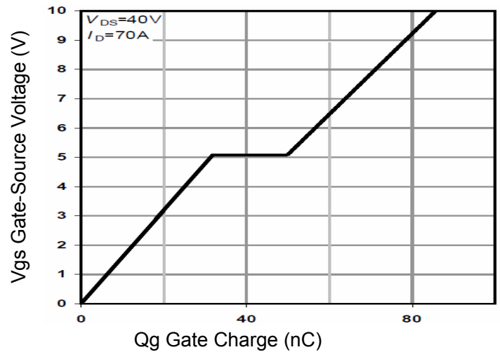
Figure 5 Gate Charge
