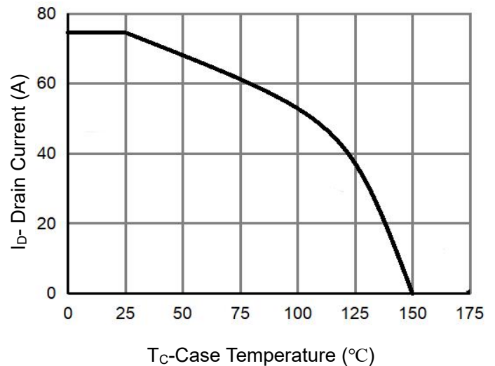
Figure 10 Current De-rating
