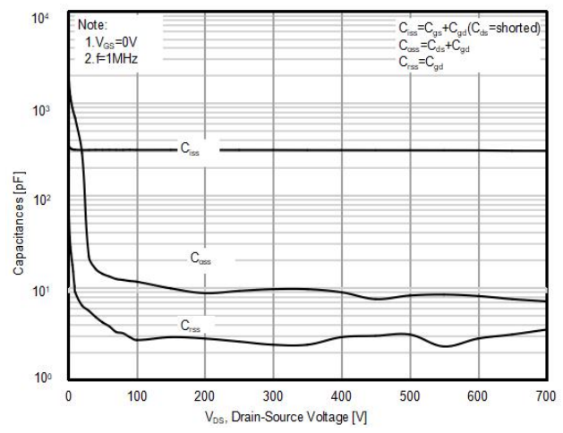
Figure10. Capacitance
