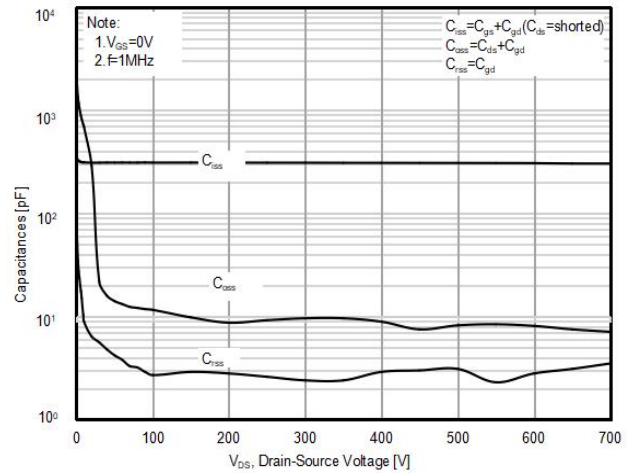
Figure10. Capacitance
