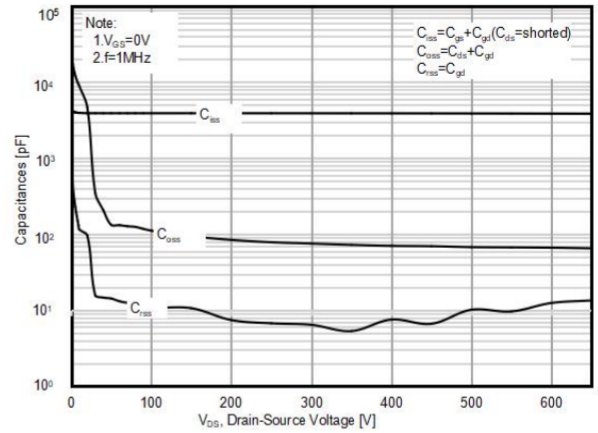
Figure2. Capacitance
