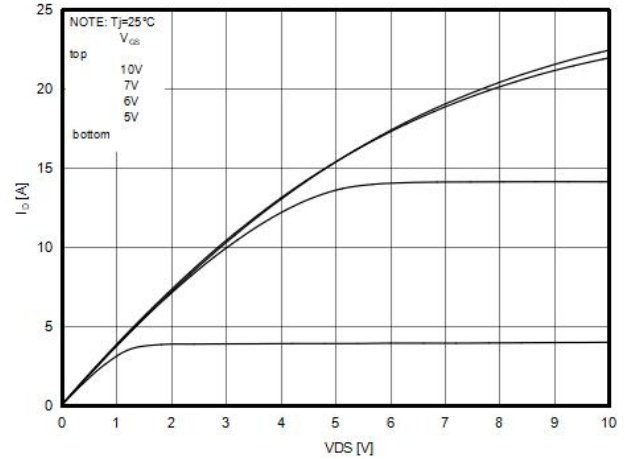
Figure4. Output characteristics
