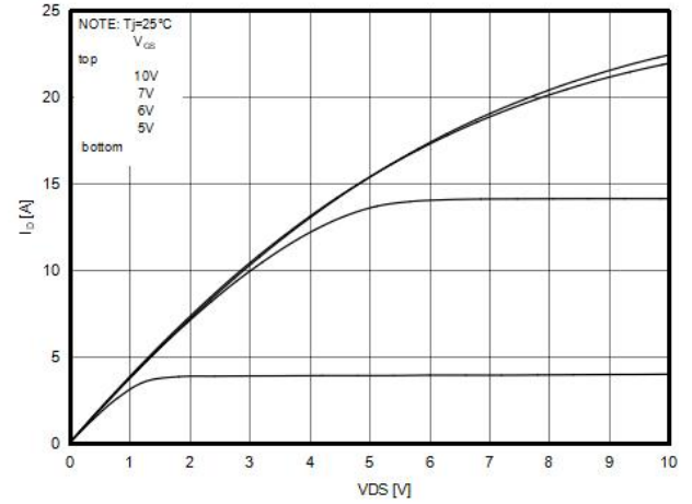
Figure4. Output characteristics
