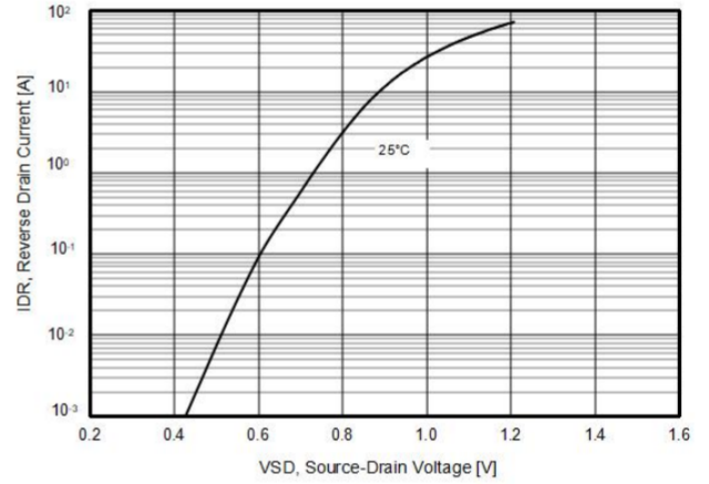
Figure10. Source-Drain Diode Forward Voltage
