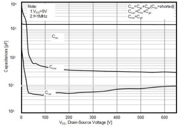
Figure2. Capacitance
