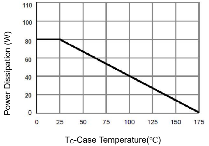
Figure 9 Power De-rating
