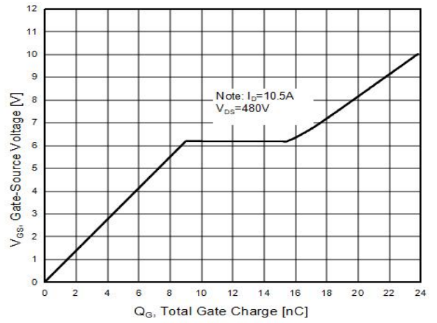
Figure8. Gate charge waveforms
