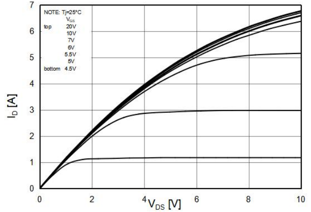
Figure4. Output characteristics
