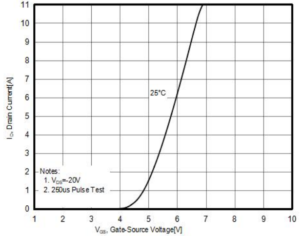
Figure4. Transfer characteristics
